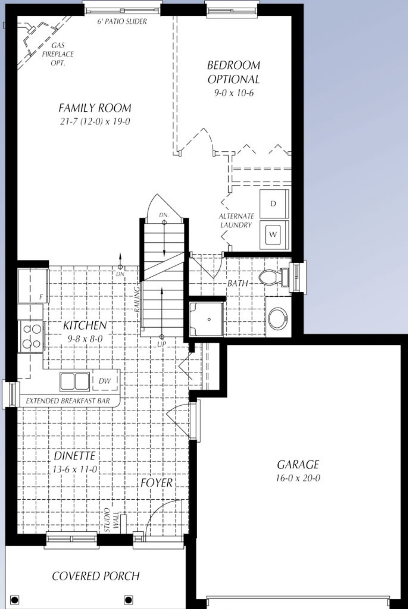
MAIN FLOOR PLAN Solar Series
