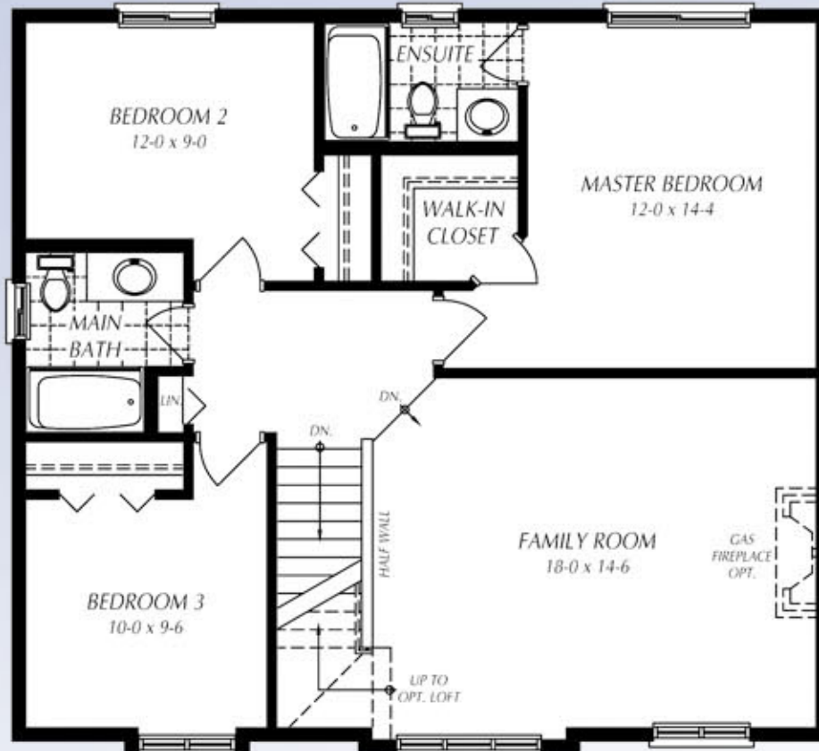
SECOND FLOOR PLAN Solar Series
