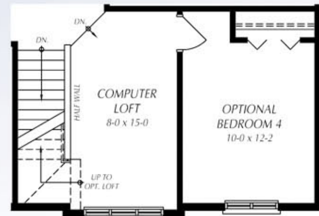
OPTIONAL 4 BEDROOM LAYOUT Solar Series
