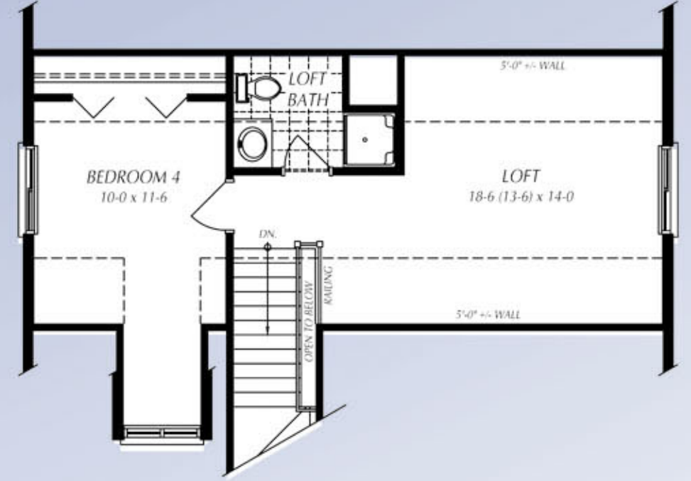
OPTIONAL LOFT FLOOR PLAN Solar Series
