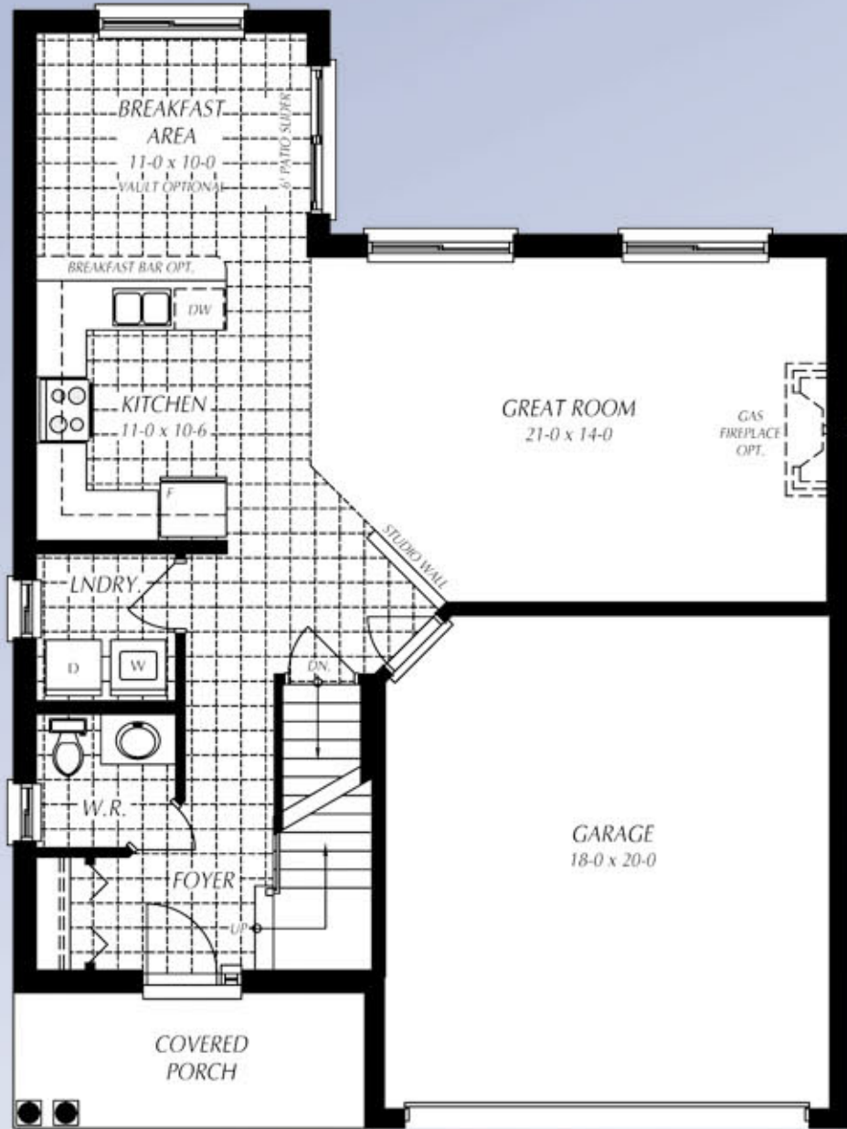
MAIN FLOOR PLAN
