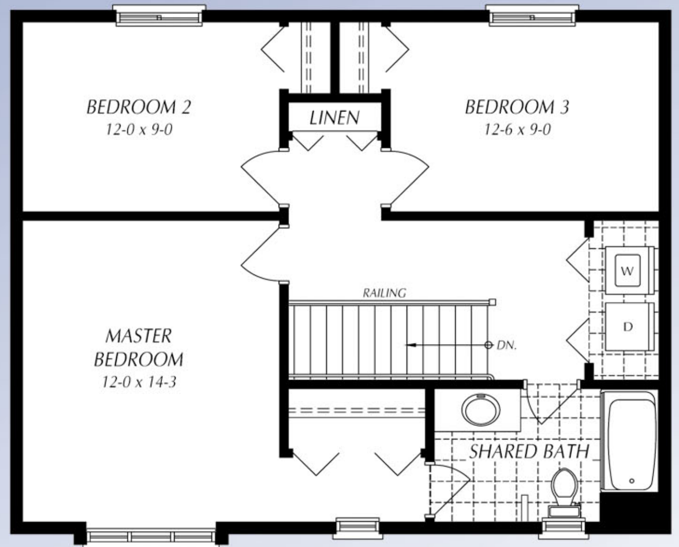
SECOND FLOOR PLAN Galaxy Series
