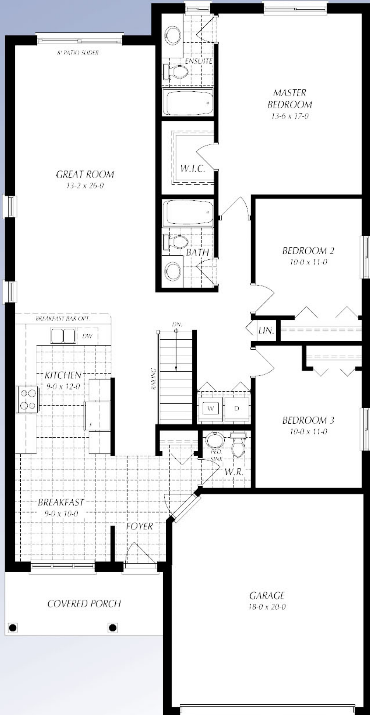
MAIN FLOOR PLAN
