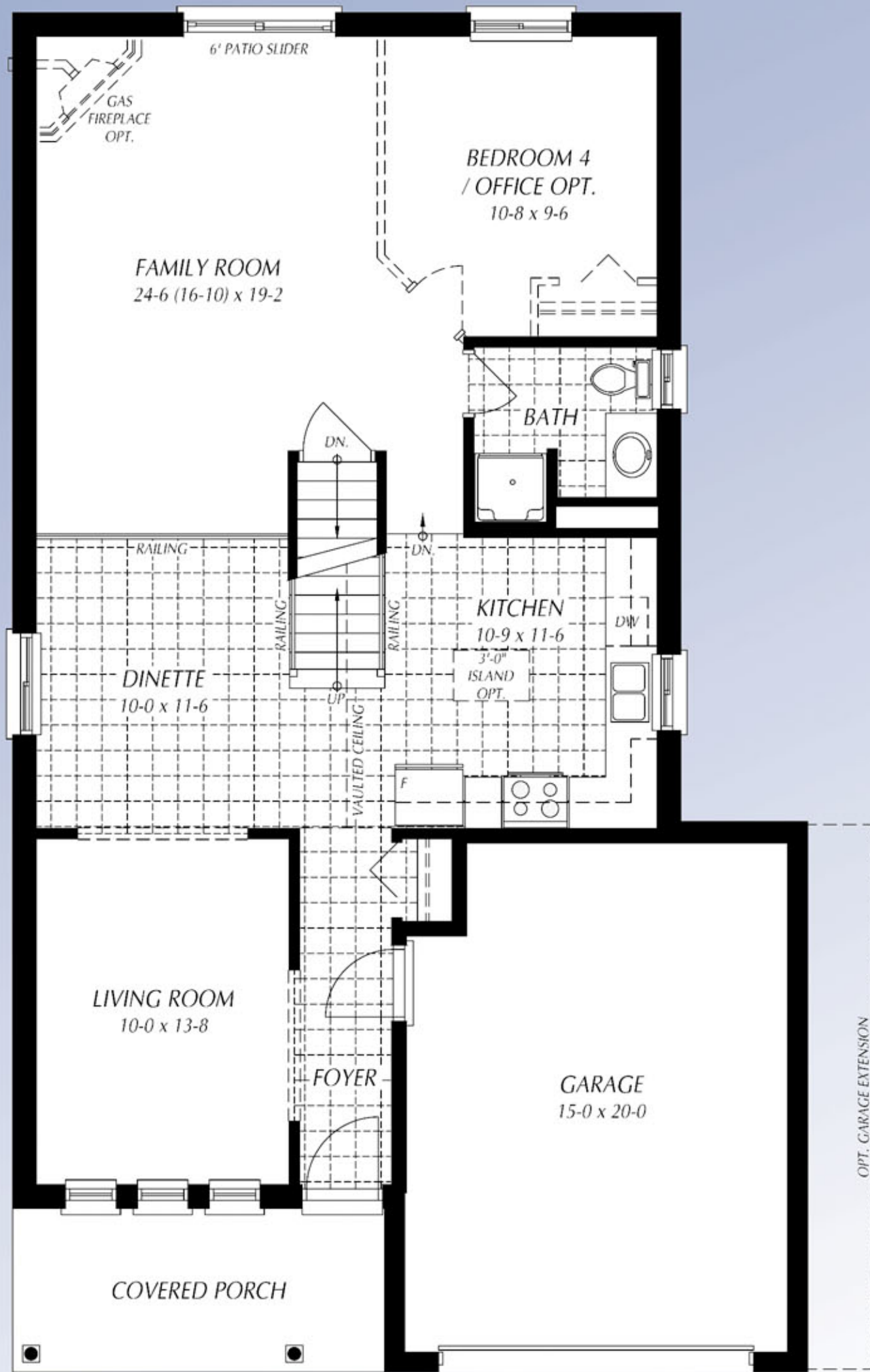
MAIN FLOOR PLAN Galaxy Series
