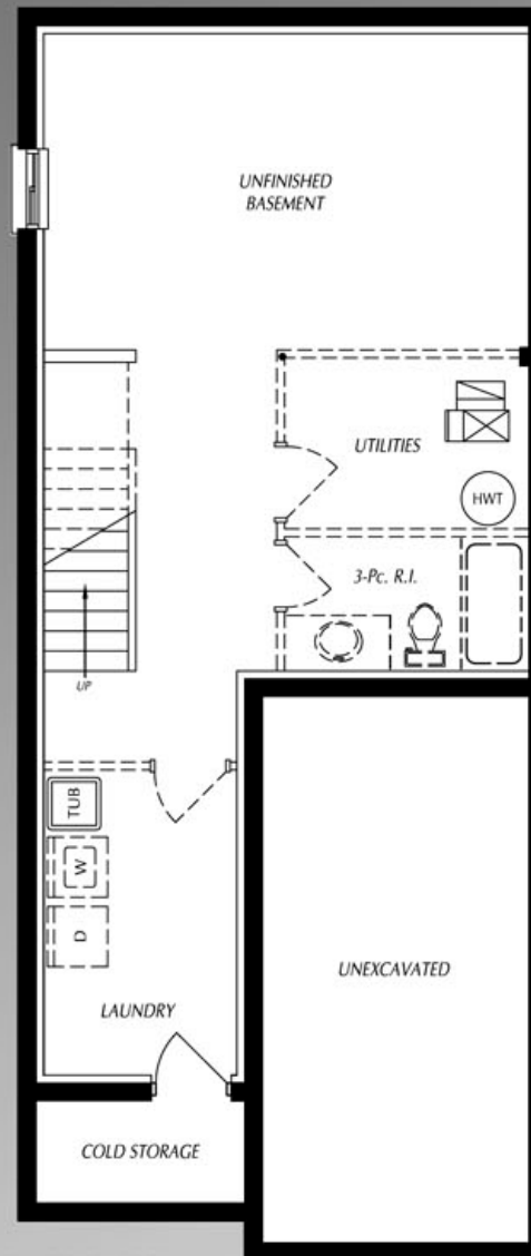
BASEMENT PLAN
