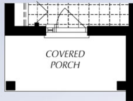
PARTIAL MAIN FLOOR PLAN Galaxy Series
