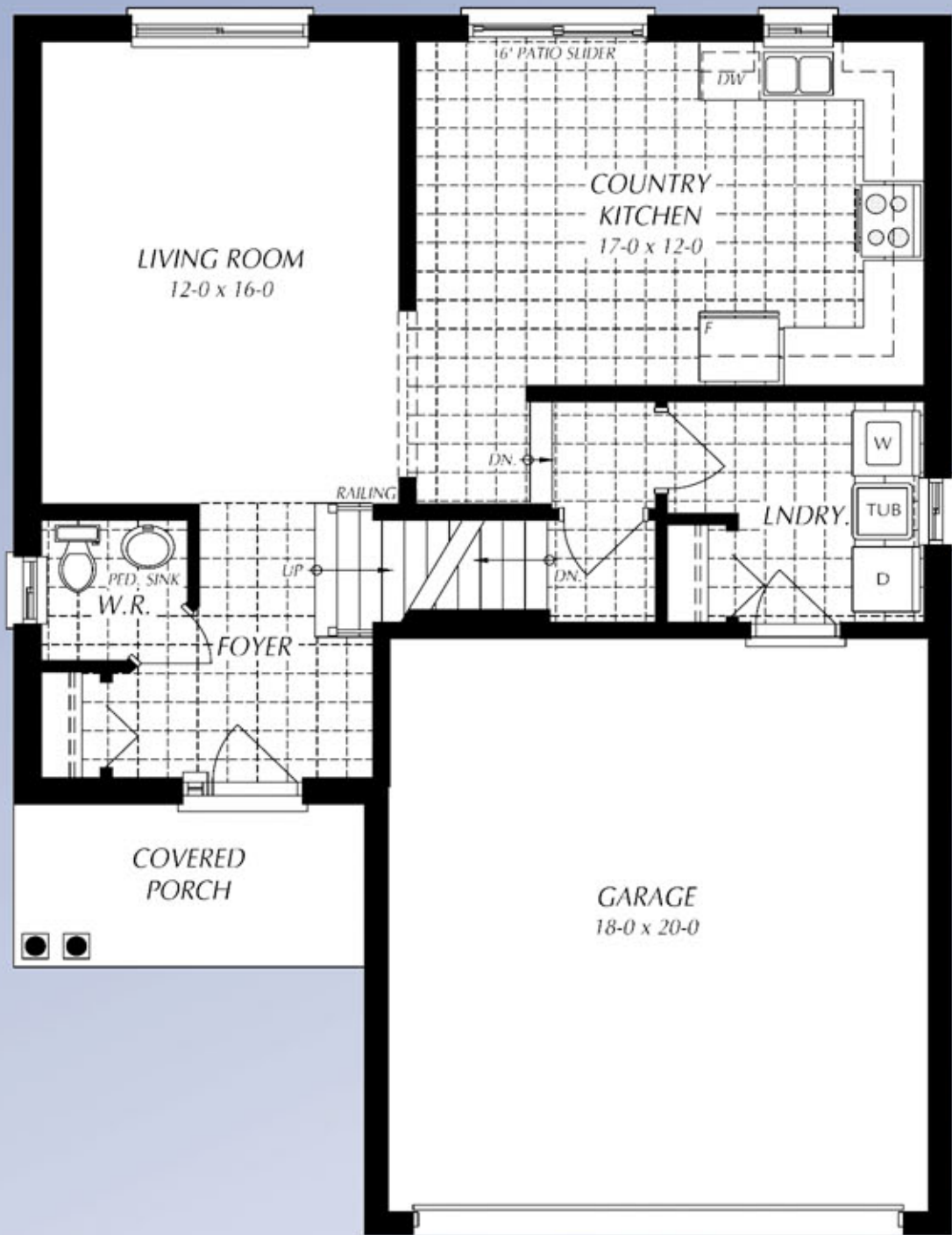
MAIN FLOOR PLAN Solar Series
