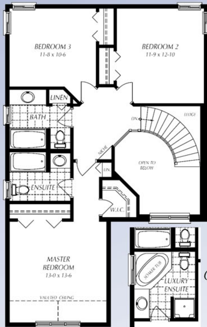
SECOND FLOOR PLAN 3 BEDROOM OPT. Solar Series
