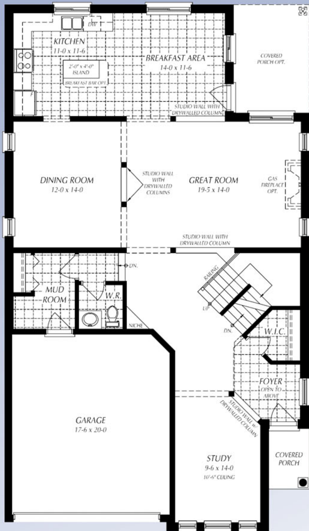
MAIN FLOOR PLAN Galaxy Series
