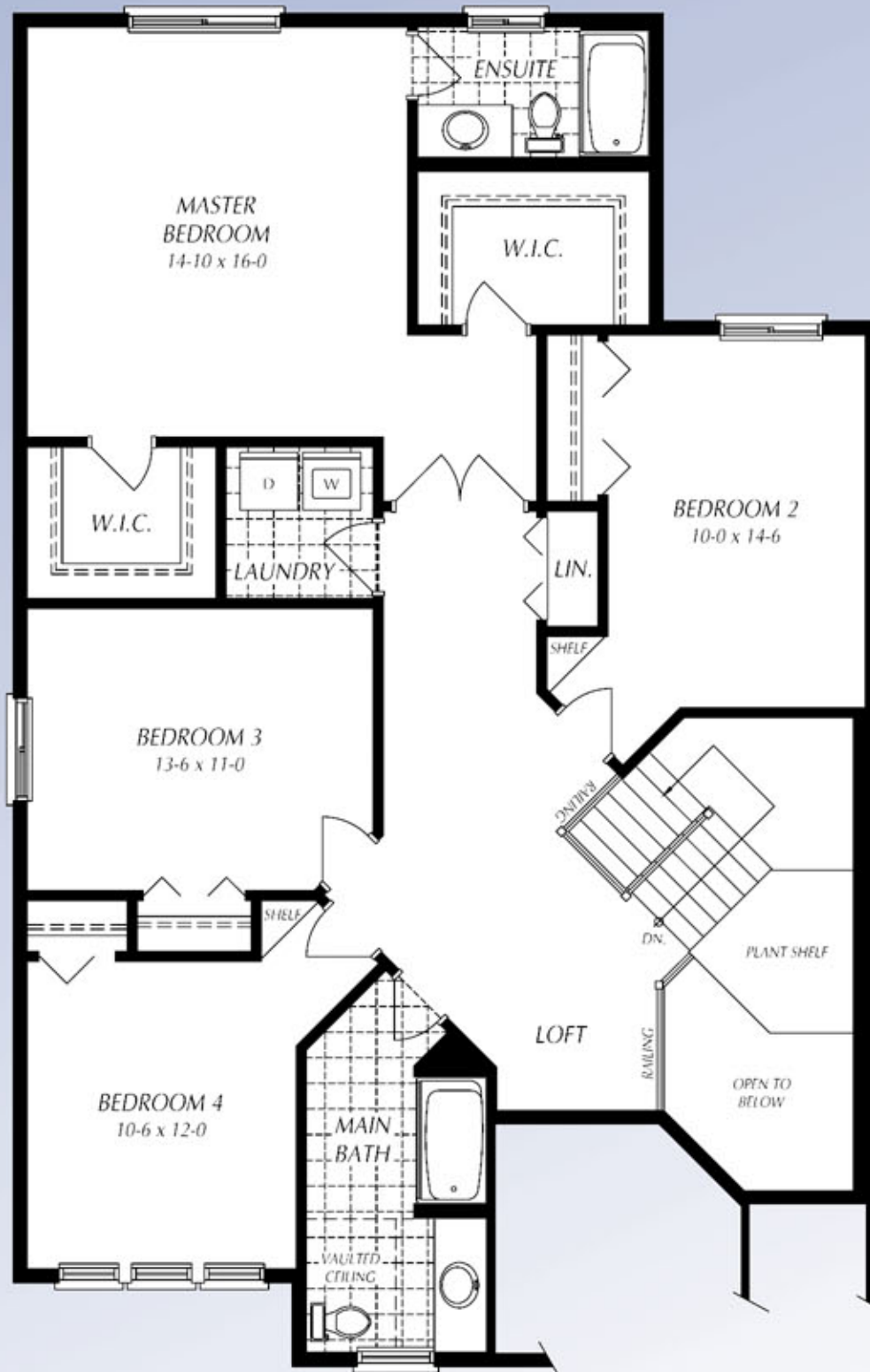
SECOND FLOOR PLAN Galaxy Series
