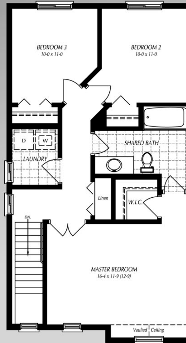
STANDARD SECOND FLOOR PLAN Galaxy Series
