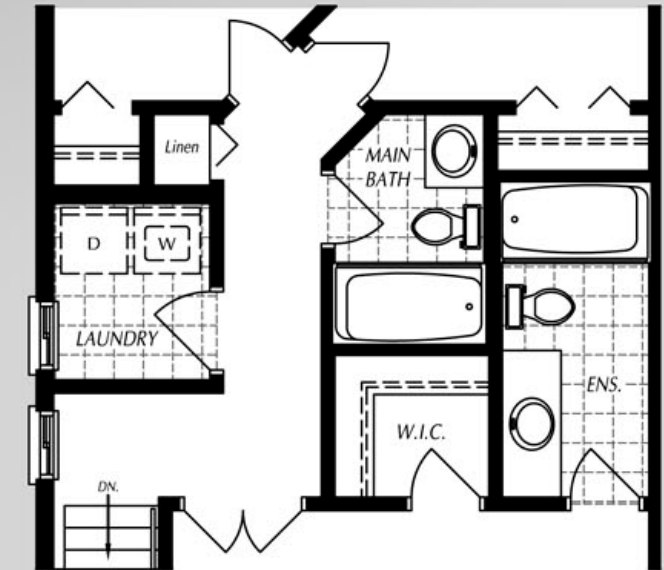
OPTIONAL SECOND FLOOR PLAN w/ Ensuite
